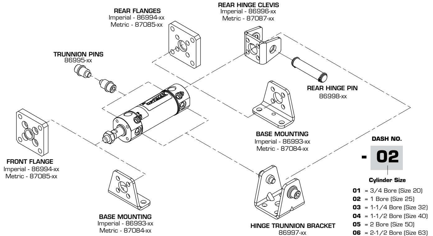
Mounting Attachments
